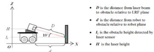
Figure 2: Laser beam decomposition in zx surface.
