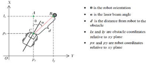
Figure 3: Laser beam decomposition in xy surface.
