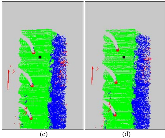
Figure 5: Mapping a path with low grass in the side. (a)Environment picture; (b)3D map of the environment; (c)Classified network using 4 hidden units and (d)using 32 units. Green color corresponds to navigable terrain, red color corresponds to the non-navigable terrain, and blue color corresponds to partially navigable terrain.
