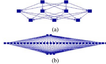
Figure 4: Neural networks used in terrain classification. (a)ANN with 4 hidden units; (b)ANN with 32 hidden units.
