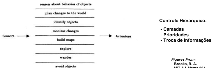
Figure 1. A traditional decomposition of a mobile robot control system into functional
